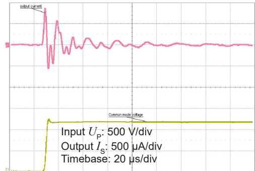
Figure 12: Detail of typical common mode perturbation (1200 V step with 6 kV/µs, R_M = 100 \Omega )
