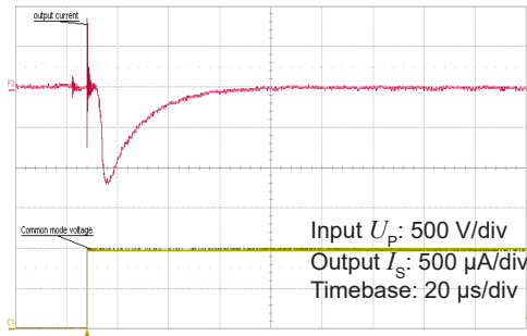
Figure 11: Typical common mode perturbation (1200 V step with 6 kV/µs R_M = 100 \Omega )
