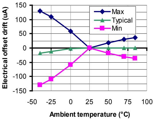
Figure 3: Electrical offset thermal drift
