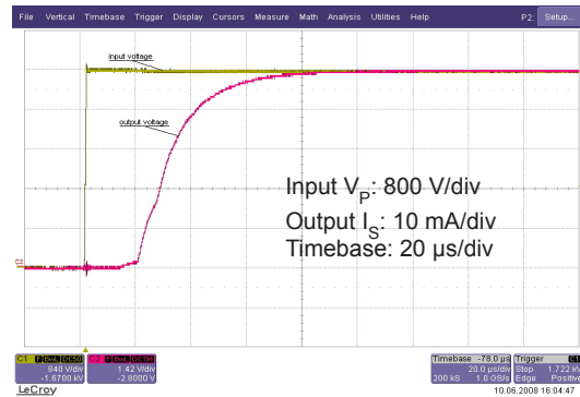
Figure 6: Typical step response (0 to 4000 V)
