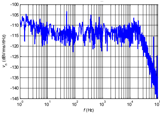
Figure 13: Typical noise power density of V_n ( R_M ) with R_M = 50 \Omega
