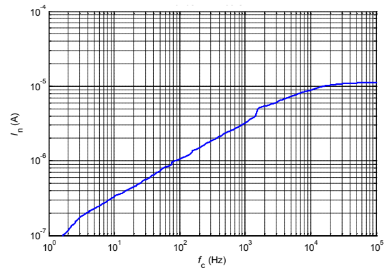
Figure 14: Typical total output current noise (rms) with R_M = 50 \Omega ( f_c is upper cut off frequency of band pass, low cut off frequency is 1 Hz)
