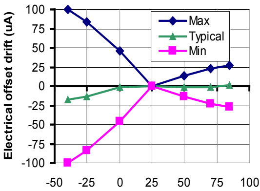
Figure 3: Electrical offset thermal drift
