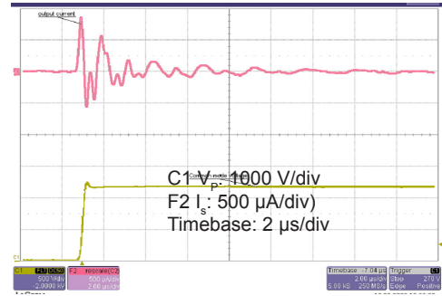
Figure 12: Detail of typical common mode perturbation (4200 V step with 6 kV/μs, R_M = 100 \Omega )
