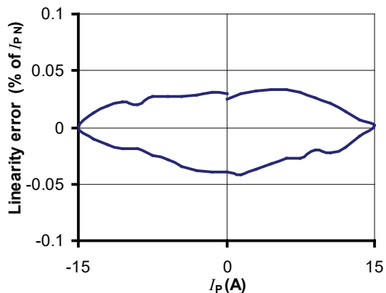
Figure 1: Linearity error
