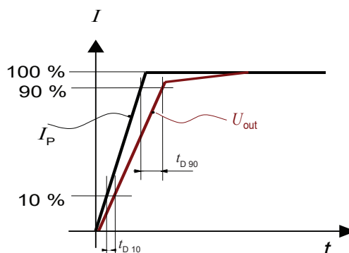
Figure 25: t_{D90} ( delay time @ 90 %) and t_{D10} ( delay time @ 10 %)
