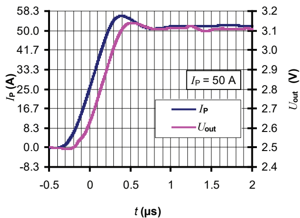
Figure 15: Step response
