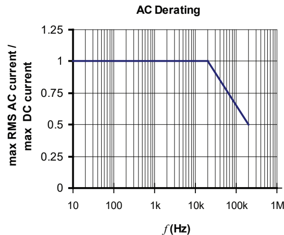
Figure 22: Maximum RMS AC primary current / maximum DC primary current vs frequency
