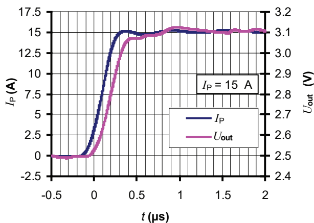
Figure 3: Step response
