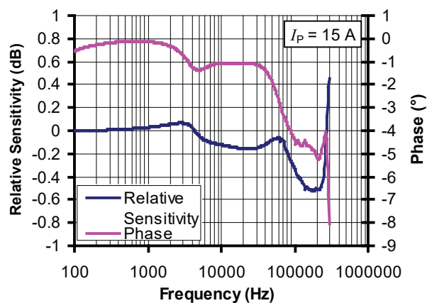
Figure 2: Frequency response
