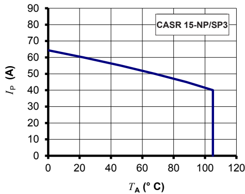
Figure 19: I_P vs T_A for CASR 15-NP/SP3
