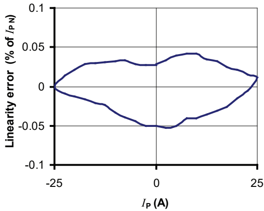
Figure 7: Linearity error
