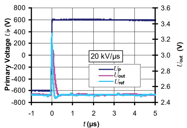
Figure 12: du/dt
