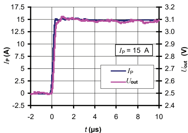
Figure 4: Step response
