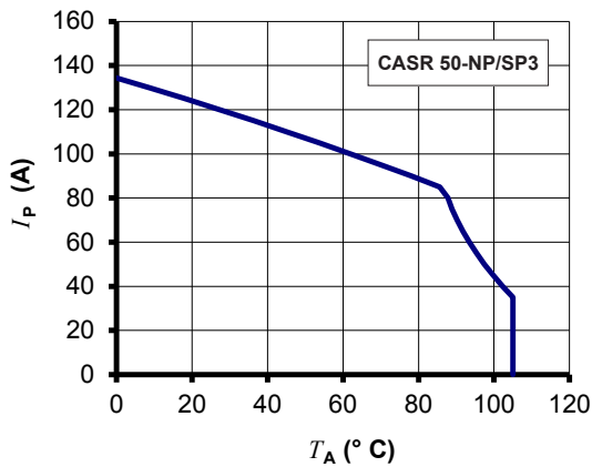
Figure 21: I_P vs T_A for CASR 50-NP/SP3
