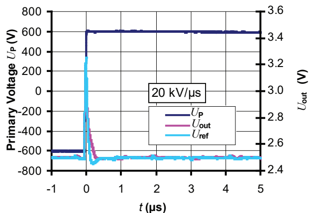
Figure 18: du/dt
