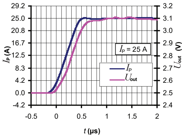
Figure 9: Step response
