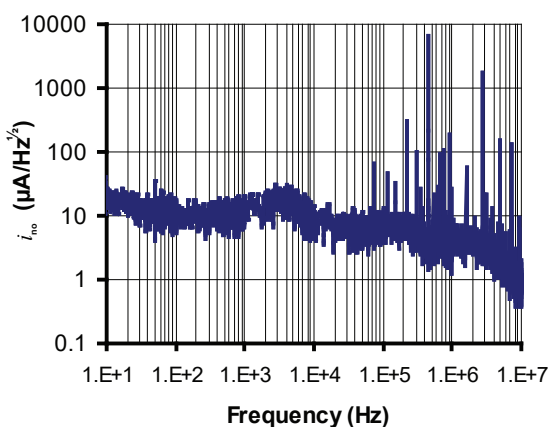
Figure 11: Noise current spectral density referred to primary
