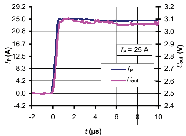
Figure 10: Step response
