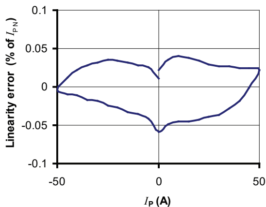
Figure 13: Linearity error
