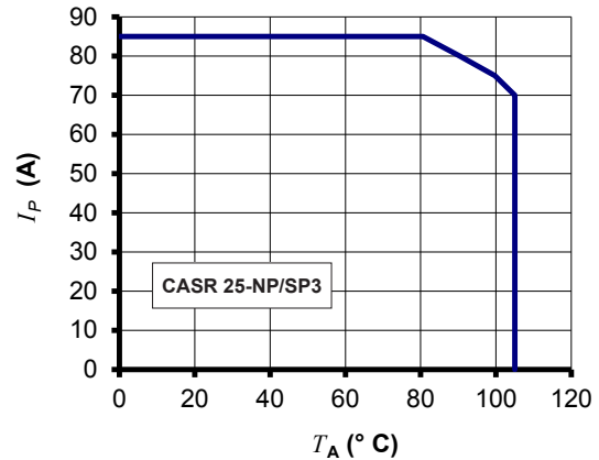
Figure 20: I_P vs T_A for CASR 25-NP/SP3
