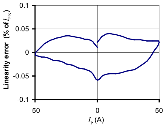
Figure 7: Linearity error
