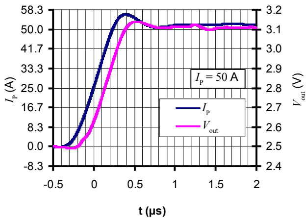
Figure 9: Step response
