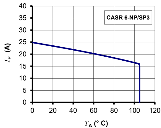
Figure 7: I_P vs T_A for CASR 6-NP/SP3
