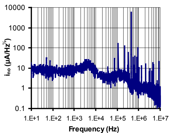
Figure 5: Output noise current
