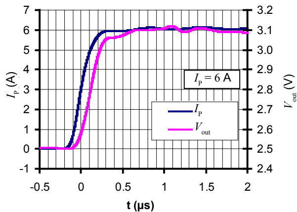
Figure 3: Step response
