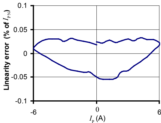
Figure 1: Linearity error
