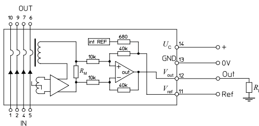
Figure 10: Test connection
