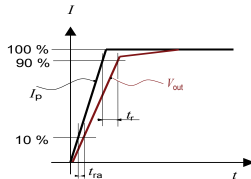
Figure 11: Response time t_r and reaction time t_{ra}
