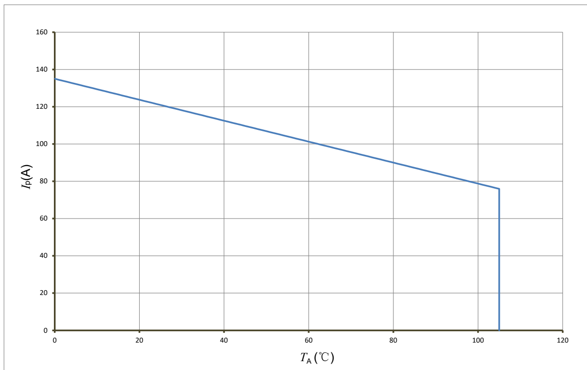
Figure 1: I_p vs T_A for CKSR 75-NP/SP1
