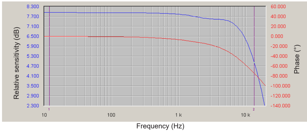
Figure 6: Frequency response
