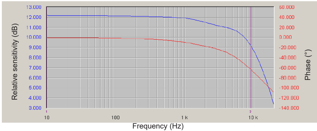
Figure 1: Frequency response
