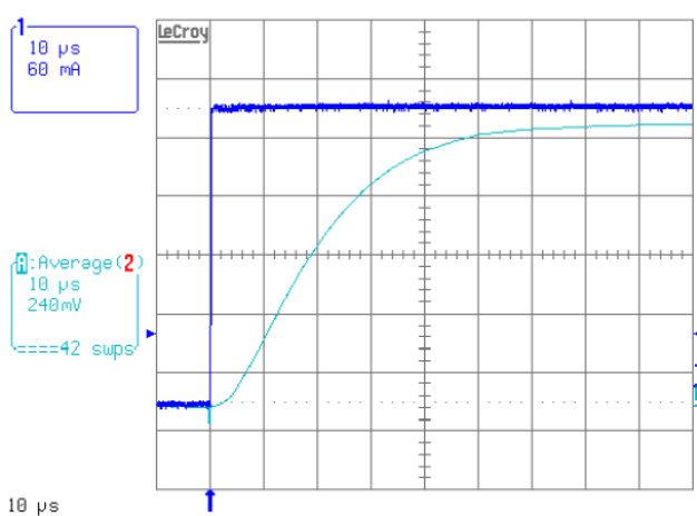
Figure 4: Typical step response
