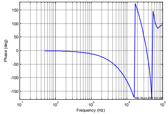
Figures 9, 10: Typical frequency response
