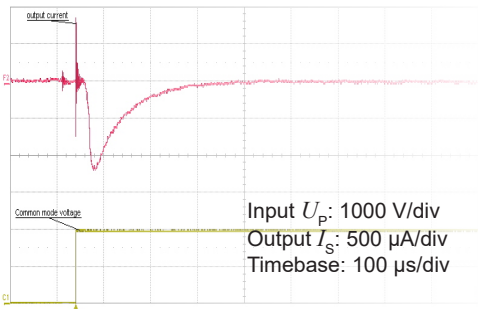
Figure 11: Typical common mode perturbation (4200 V step with 6 kV/μs R_M = 100 \Omega )
