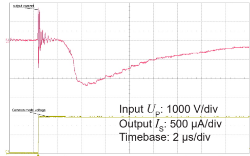
Figure 12: Detail of typical common mode perturbation (4200 V step with 6 kV/μs, R_M = 100 \Omega )
