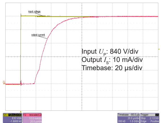
Figure 6: Typical step response (0 to 4200 V)
