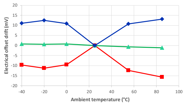
Figure 3: Electrical offset thermal drift
