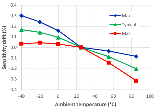
Figure 4: Sensitivity thermal drift
