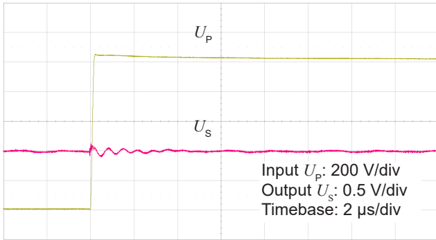
Figure 6: Detail of typical common mode perturbation (1000 V step with 6 kV/μs)
