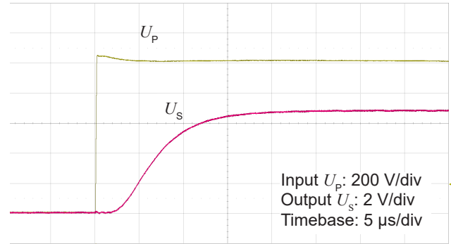
Figure 7: Typical delay time (0 to 1000 V)
