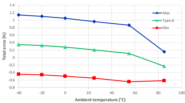
Figure 2: Total error in temperature
