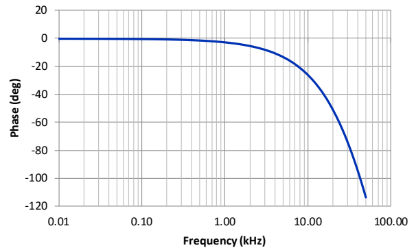
Figure 9: Phase shift function of frequency
