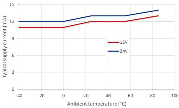
Figure 1: Supply current function of temperature
