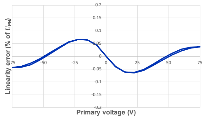
Figure 6: Typical linearity error at 25 °C
