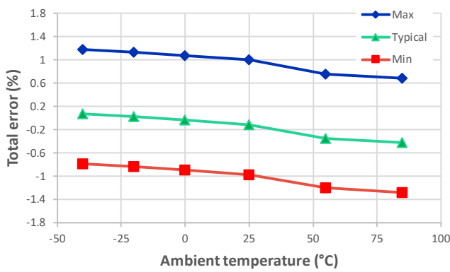
Figure 3: Total error in temperature
