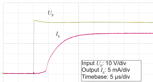
Figure 8: Typical step response (0 to 50 V)
