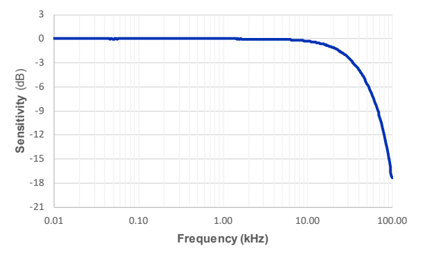
Figure 9: Sensitivity function of frequency
