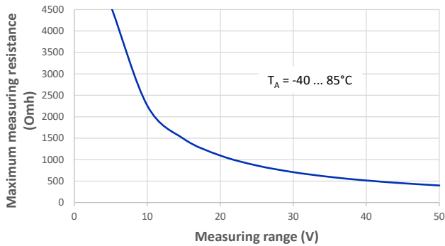
Figure 1: Maximum measuring resistance
