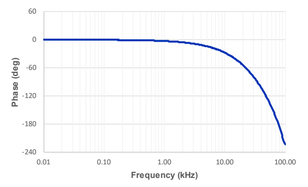
Figure 10: Phase shift function of frequency
