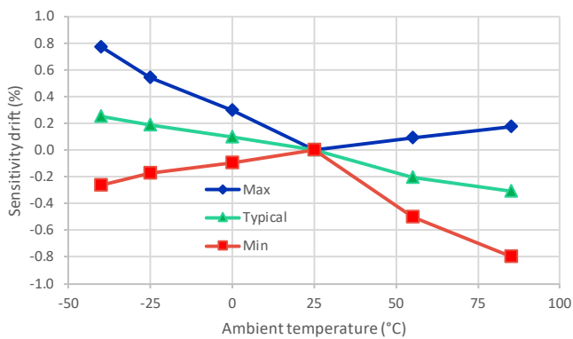
Figure 5: Sensitivity thermal drift
