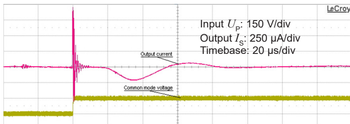
Figure 14: Detail of typical common mode perturbation (150 V step with 6 kV/μs, R_M = 100 \Omega )
