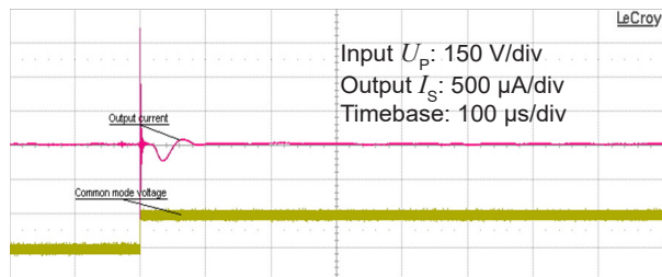
Figure 13: Typical common mode perturbation (150 V step with 6 kV/μs R_M = 100 \Omega )
