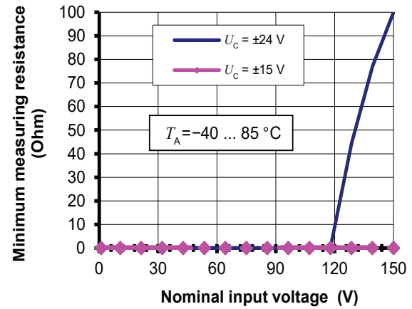
Figure 2: Minimum measuring resistance For T_A under 80 \text{ } ^\circ\text{C} , the minimum measuring resistance is 0 \text{ } \Omega whatever U_C
