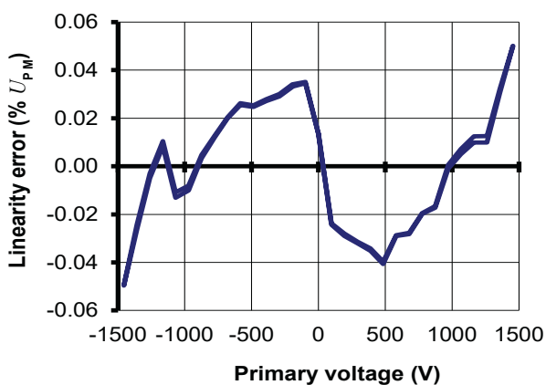
Figure 17: Typical linearity error at 25^\circ\text{C}
