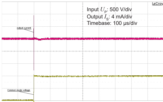
Figure 13: Typical common mode perturbation (1000 V step with 6 \text{ kV}/\mu\text{s} , R_M = 100 \Omega )
