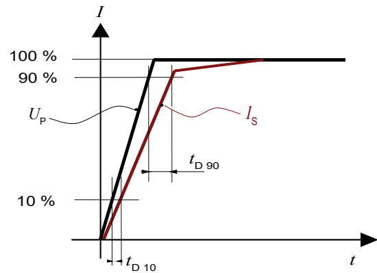
Figure 19: Delay time t_{D90} @ 90 and delay time t_{D10} @ 10
