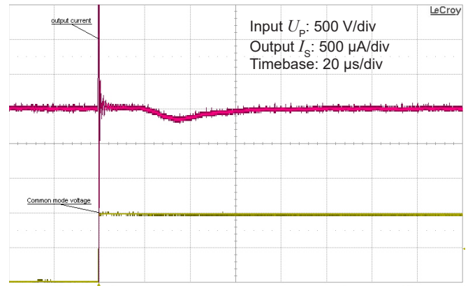
Figure 14: Detail of typical common mode perturbation (1000 V step with 6 \text{ kV}/\mu\text{s} , R_M = 100 \Omega )
