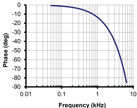
Figure 11 and 12: Typical frequency and phase response (detail)
