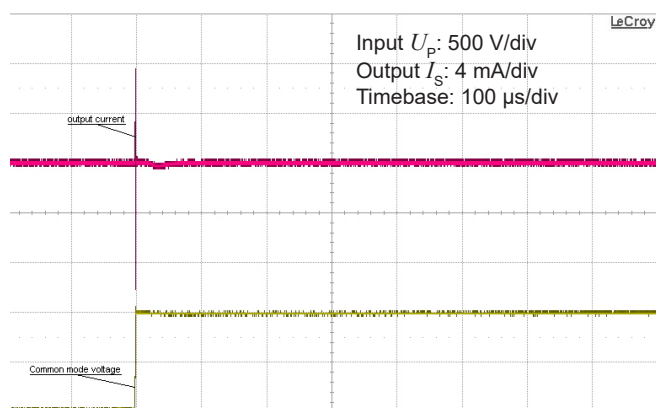
Figure 13: Typical common mode perturbation (1000 V step with 6 kV/μs, R_M = 100 \Omega )
