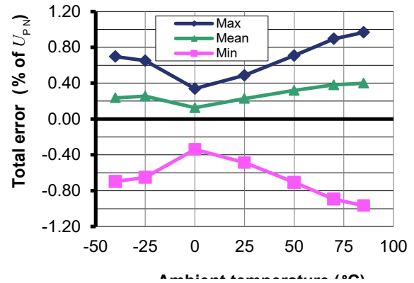
Figure 4: Total error in temperature
