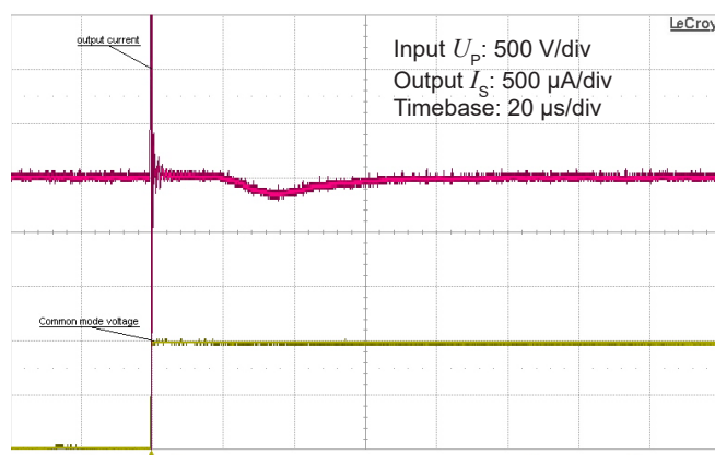
Figure 14: Detail of typical common mode perturbation (1000 V step with 6 kV/μs, R_M = 100 \Omega )
