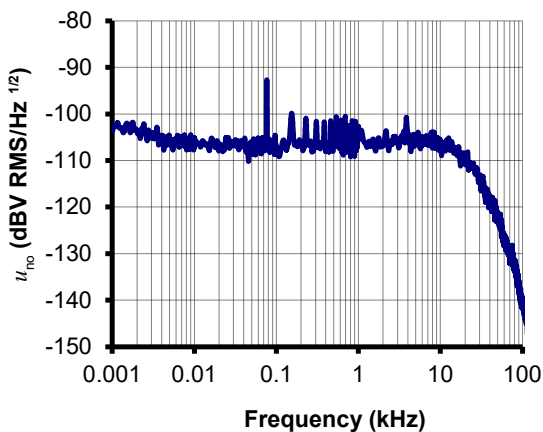
Figure 15: Typical noise voltage spectral density of u_{no} with R_M = 50 \Omega
