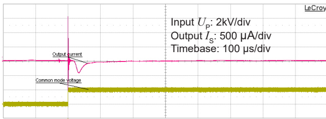
Figure 13: Typical common mode perturbation (125 V step with 6 kV/μs R_M = 100 \Omega )
