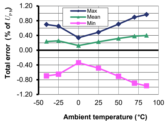
Figure 4: Total error in temperature
