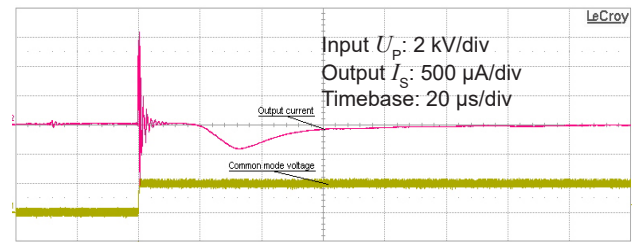
Figure 14: Detail of typical common mode perturbation (125 V step with 6 kV/μs, R_M = 100 \Omega )
