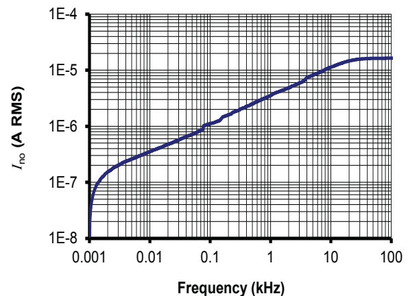
Figure 16: Typical total output RMS noise current with R_M = 50 \Omega ( f_c is upper cut-off frequency of bandpass, low cut off frequency is 1 Hz)
