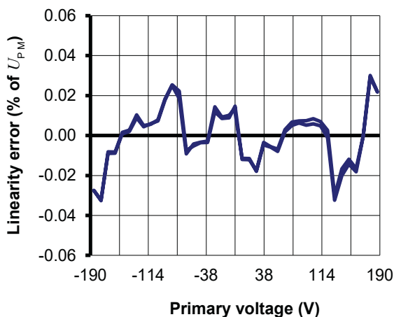
Figure 17: Typical linearity error at 25 °C
