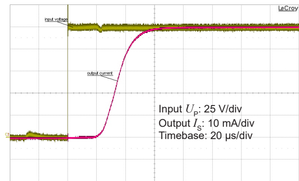
Figure 6: Typical step response (0 to 125 V)
