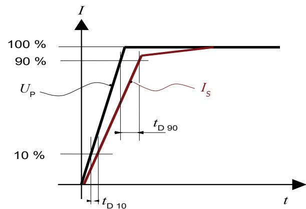
Figure 19: Delay time t_{D90} @ 90 and delay time t_{D10} @ 10
