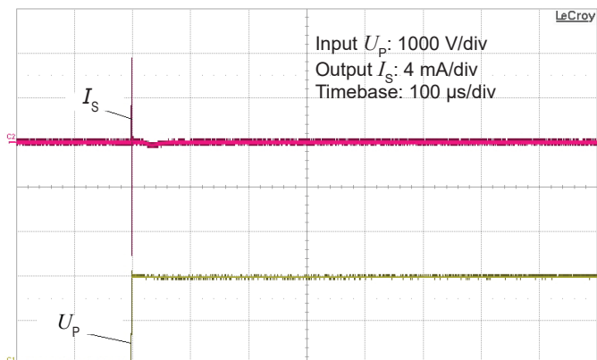
Figure 13: Typical common mode perturbation (2000 V step with 6 \text{ kV}/\mu\text{s} , R_M = 100 \Omega )
