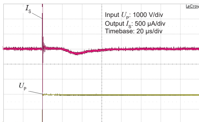
Figure 14: Detail of typical common mode perturbation (2000 V step with 6 \text{ kV}/\mu\text{s} , R_M = 100 \Omega )
