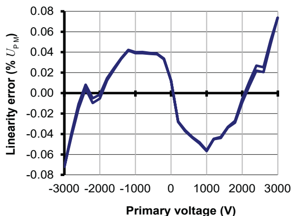
Figure 17: Typical linearity error at 25^\circ\text{C}
