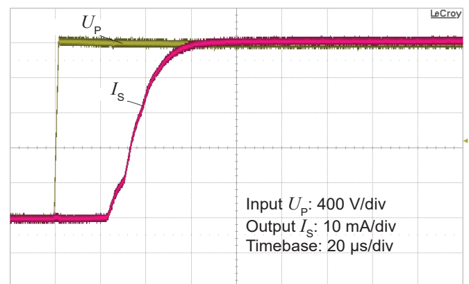
Figure 6: Typical step response (0 to 2000 V)
