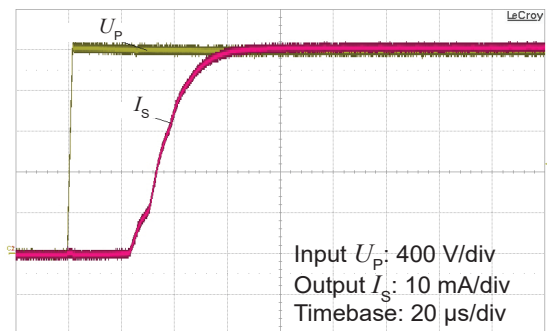
Figure 6: Typical step response (0 to 2000 V)
