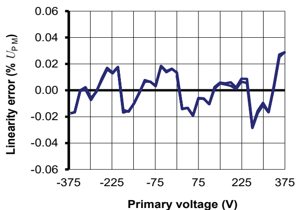
Figure 17: Typical linearity error at 25 °C
