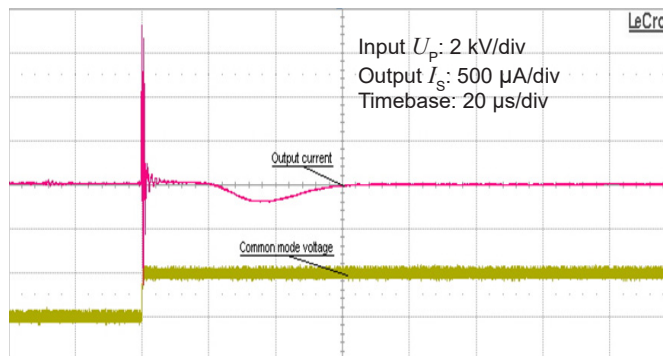
Figure 14: Detail of typical common mode perturbation (250 V step with 6 kV/μs, R_M = 100 \Omega )
