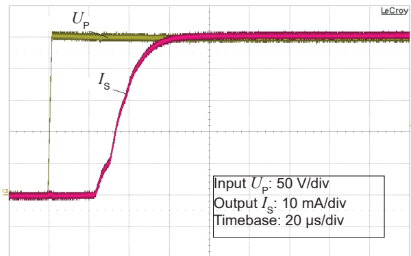
Figure 6: Typical step response (0 to 250 V)
