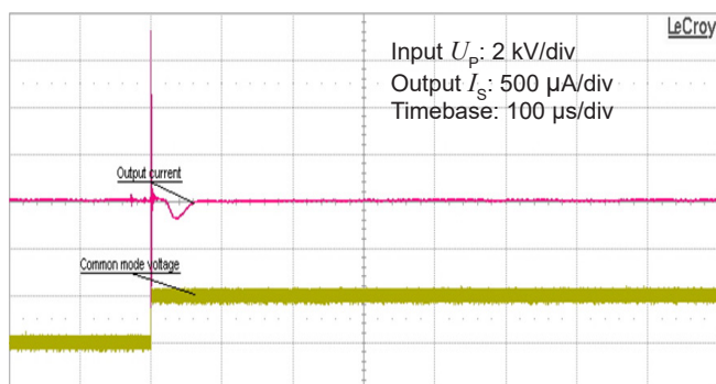
Figure 13: Typical common mode perturbation (250 V step with 6 kV/μs R_M = 100 \Omega )
