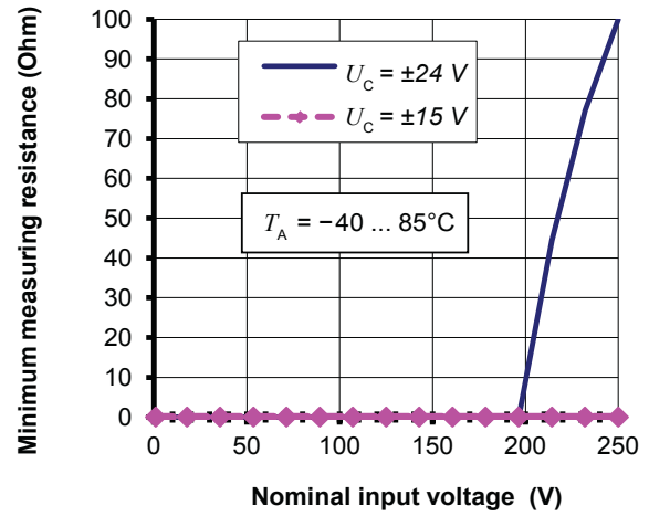
Figure 2: Minimum measuring resistance For T_A under 80^\circ\text{C} , the minimum measuring resistance is 0 \Omega whatever U_C
