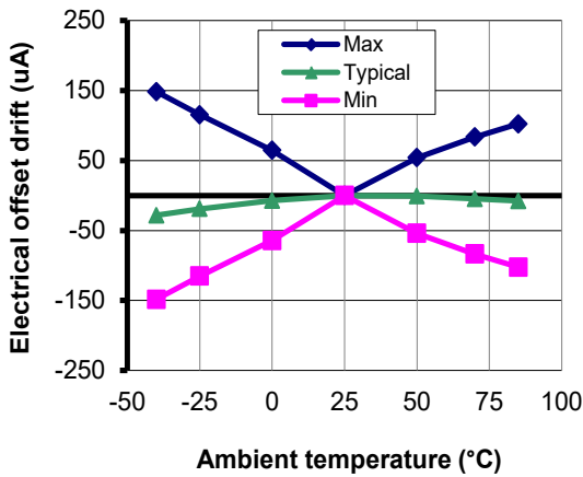
Figure 3: Electrical offset thermal drift
