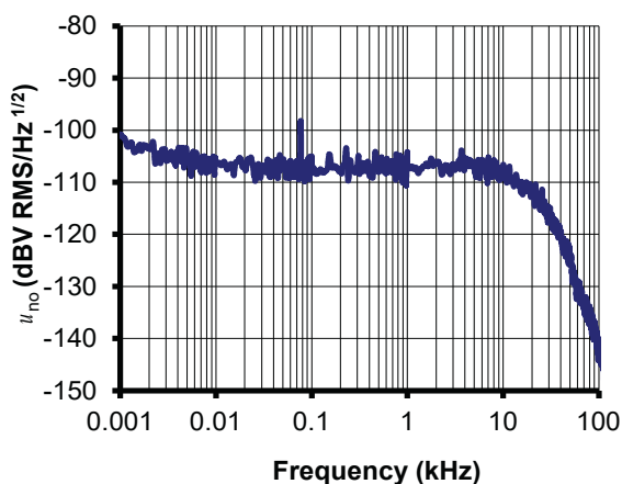
Figure 15: Typical output noise voltage spectral density u_{no} with R_M = 50 \Omega
