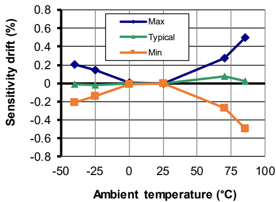
Figure 6: Sensitivity thermal drift
