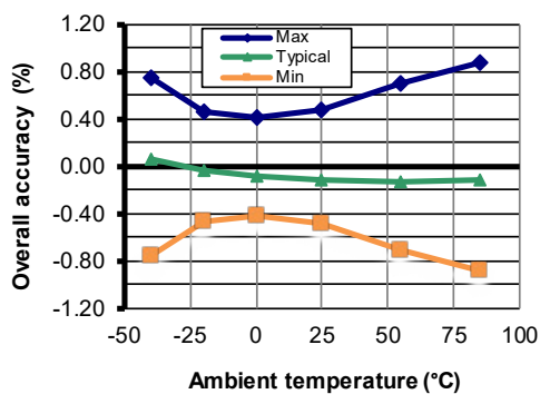
Figure 3: Total error in temperature
