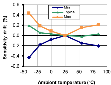
Figure 5: Sensitivity thermal drift
