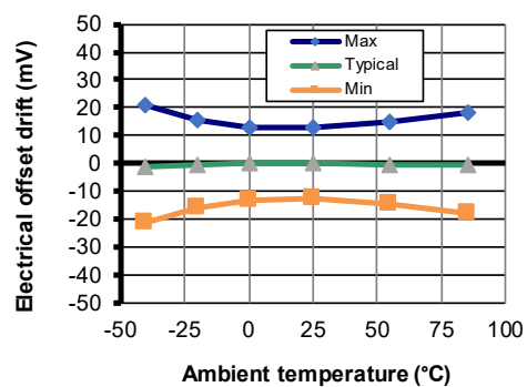
Figure 4: Electrical offset thermal drift
