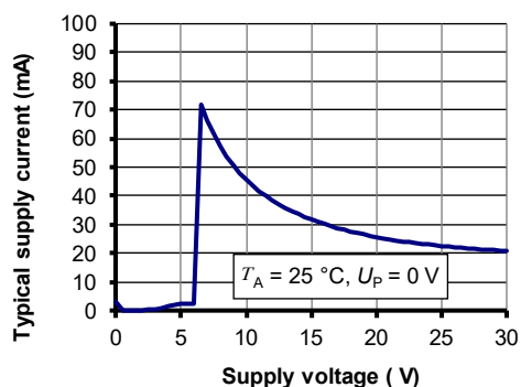
Figure 1: Supply current function of supply voltage
