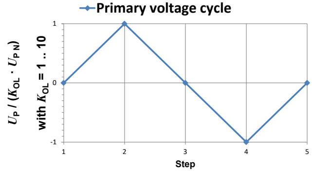
Figure 13: voltage cycle used to measure the electrical offset (transducer supplied)
