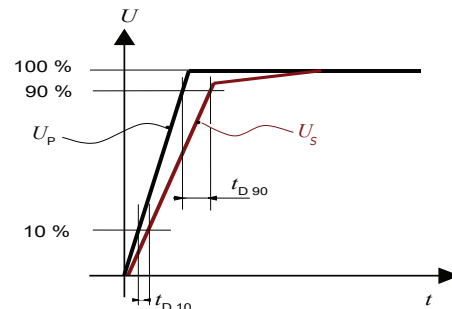
Figure 14: delay time t_{D10} @ 10 % delay time t_{D90} @ 90 %.
