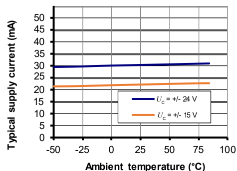
Figure 2: Supply current function of temperature
