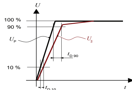
Figure 15: delay time t_{D10} @ 10 % delay time t_{D90} @ 90 %.
