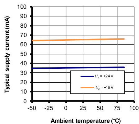
Figure 3: Supply current function of temperature
