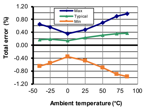
Figure 4: Total error in temperature
