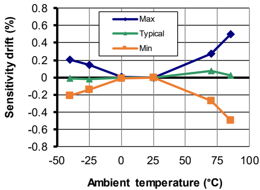
Figure 6: Sensitivity thermal drift
