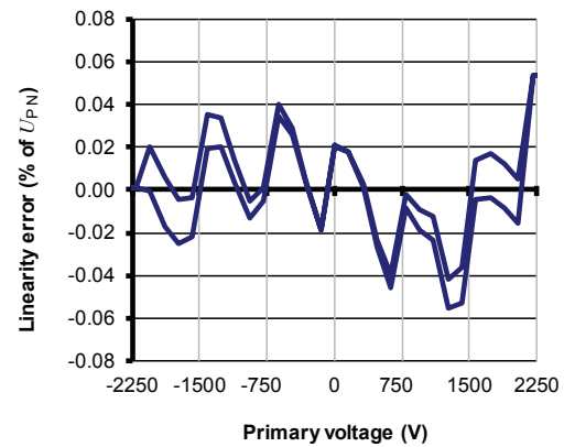
Figure 7: Typical linearity error at 25 °C
