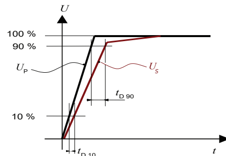
Figure 16: delay time t_{D10} @ 10 % delay time t_{D90} @ 90 %.
