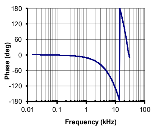
Figure 13: Phase shift function of frequency
