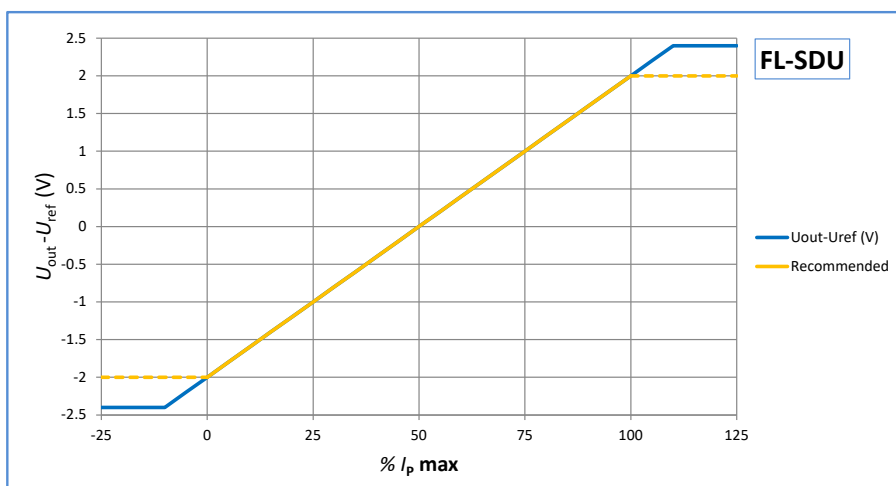
Figure 2: Uni-polar output voltage ( U_{\text{out}} - U_{\text{ref}} ) VS primary current I_p
