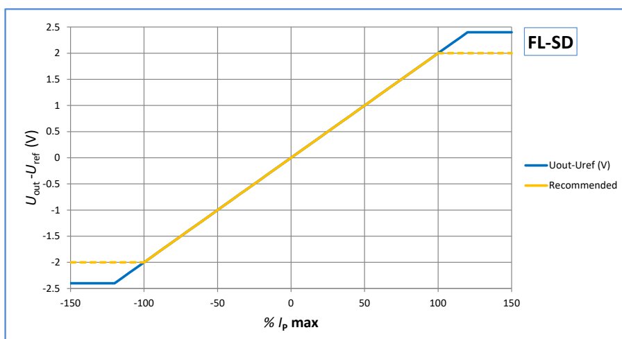
Figure 1: Bi-polar output voltage ( U_{\text{out}} - U_{\text{ref}} ) VS primary current I_p
