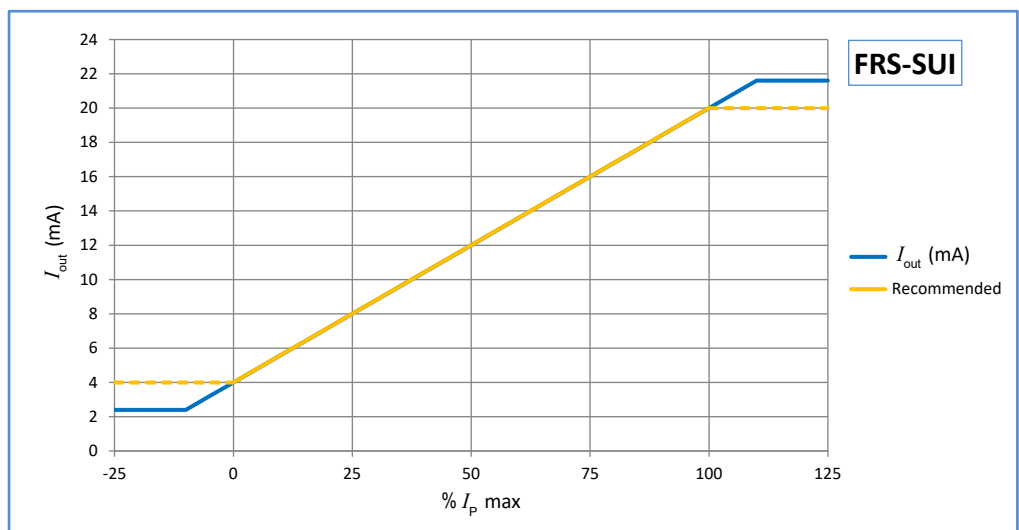
Figure 2: Uni-polar output current I_{\text{out}} VS primary current I_P
