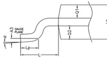
DETAIL X (Rotate -90°)
