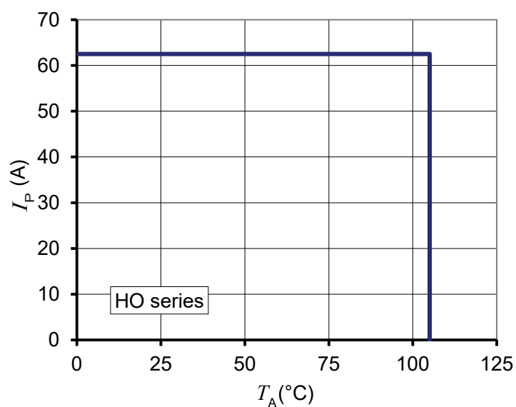
Figure 1: I_P vs T_A for HO series
