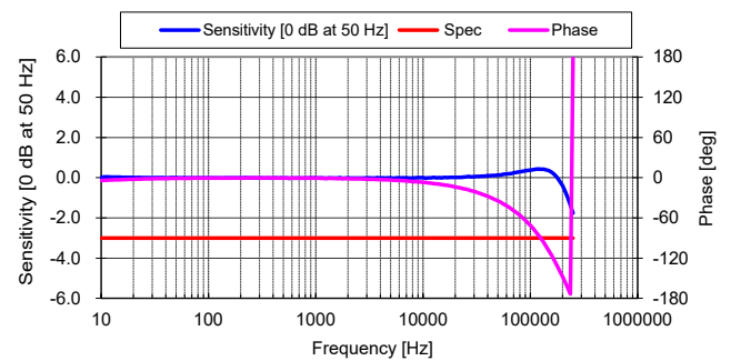
Figure 7: Frequency response
