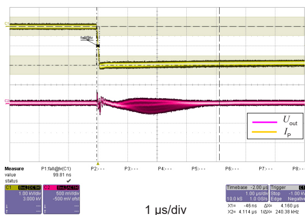
Figure 14: dv/dt
