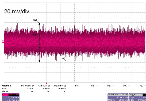
Figure 5: Output noise
