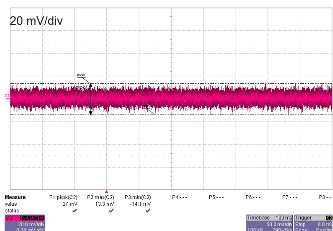
Figure 15: Output noise
