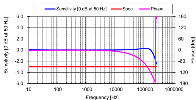
Figure 2: Frequency response
