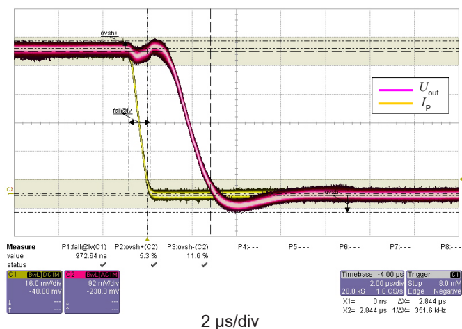
Figure 3: Step response
