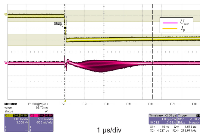
Figure 14: dv/dt
