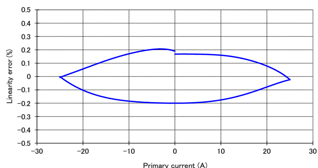
Figure 11: Linearity error
