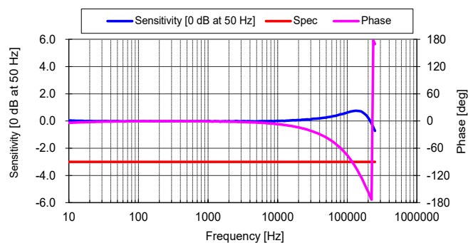
Figure 12: Frequency response
