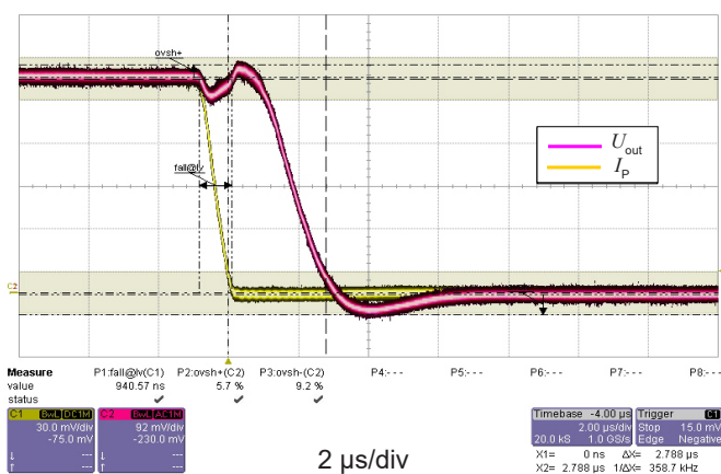
Figure 8: Step response
