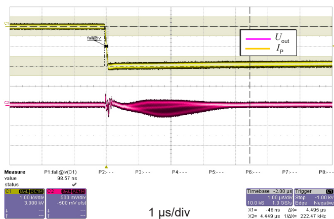
Figure 9: dv/dt
