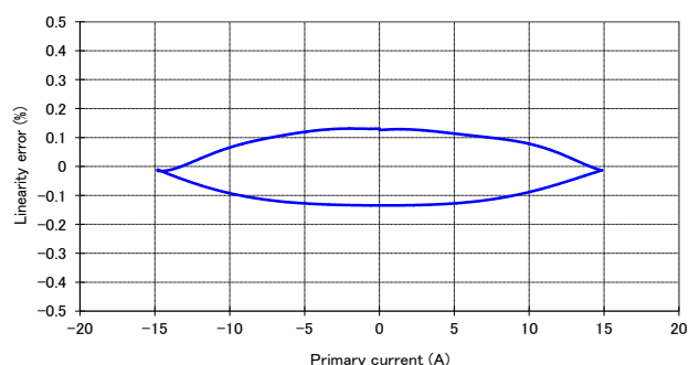
Figure 6: Linearity error
