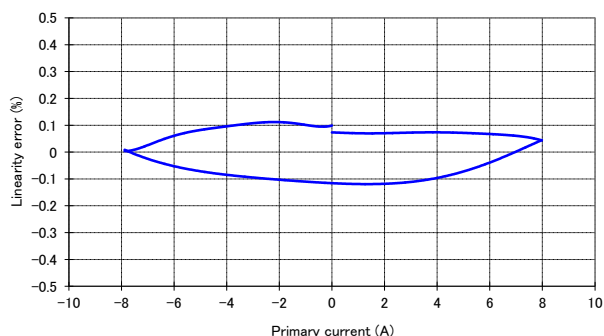
Figure 1: Linearity error
