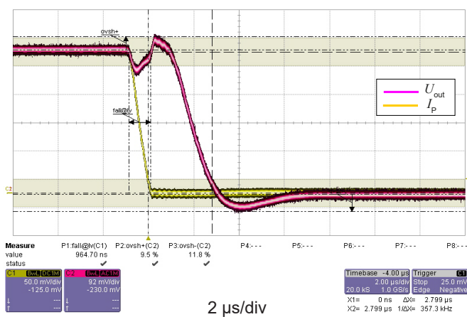
Figure 13: Step response
