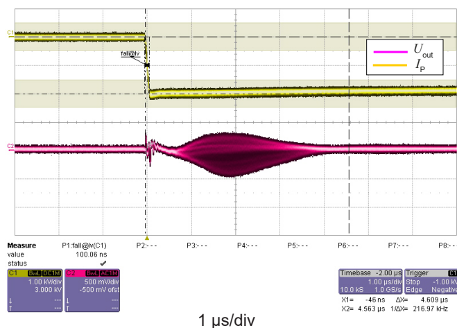
Figure 4: dv/dt
