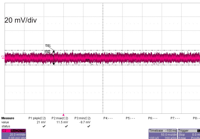
Figure 5: Output noise
