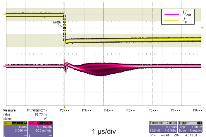
Figure 4: dv/dt
