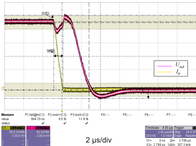
Figure 3: Step response
