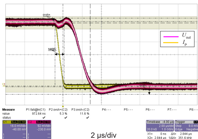
Figure 3: Step response
