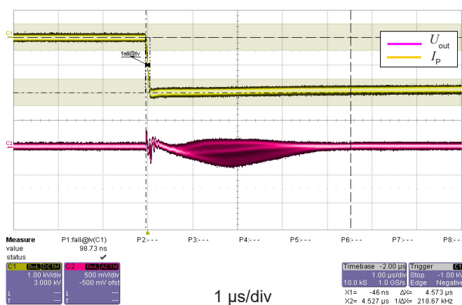
Figure 14: dv/dt
