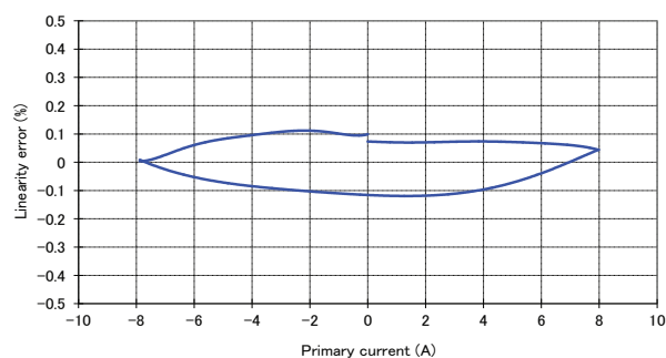
Figure 1: Linearity error
