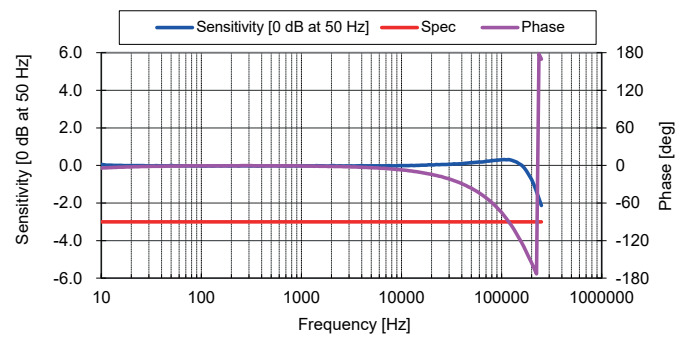
Figure 7: Frequency response
