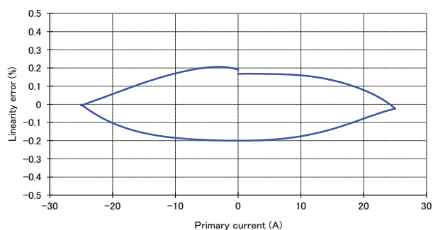
Figure 11: Linearity error
