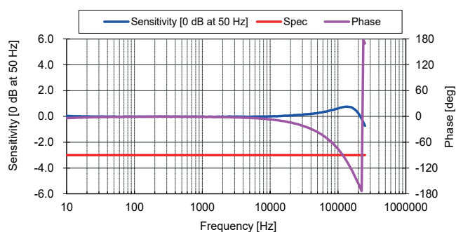
Figure 12: Frequency response
