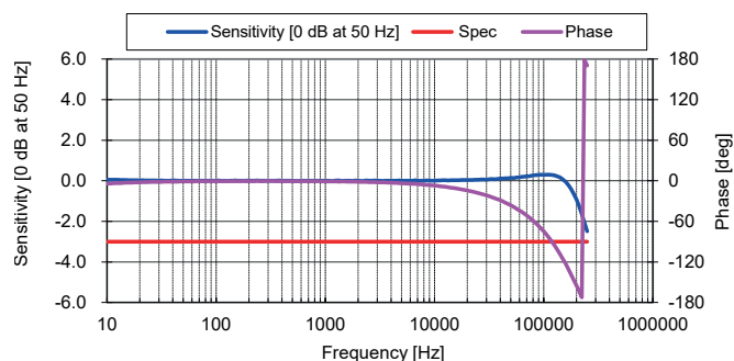
Figure 2: Frequency response
