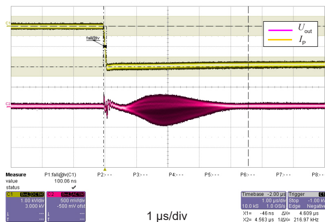
Figure 4: dv/dt
