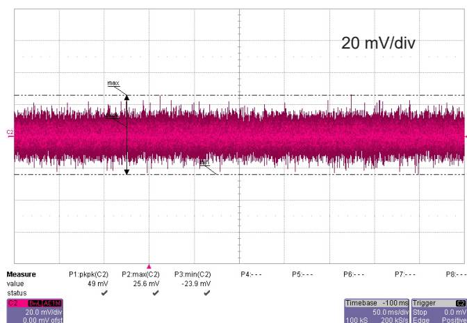
Figure 5: Output noise
