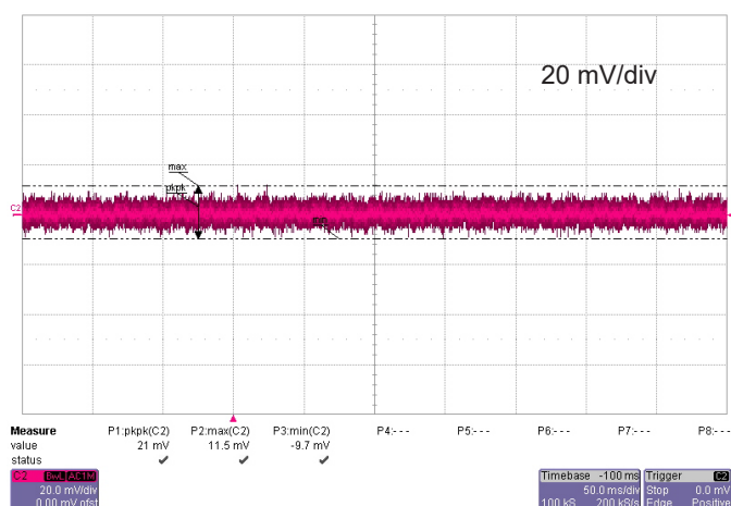
Figure 15: Output noise
