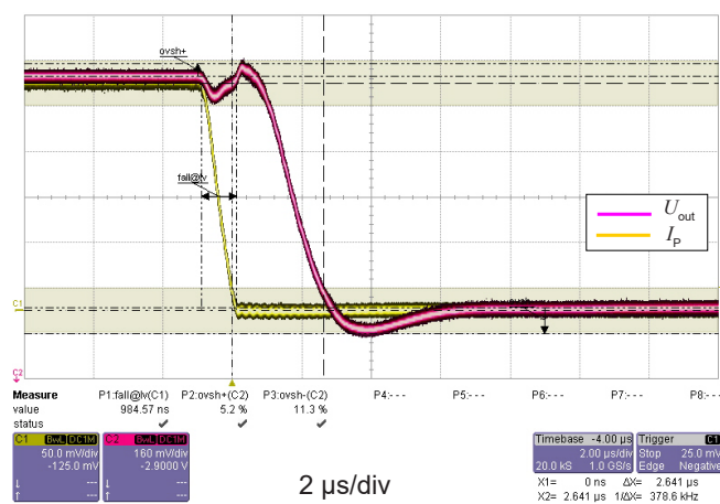
Figure 8: Step response
