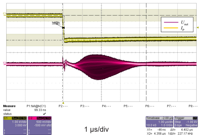
Figure 4: dv/dt
