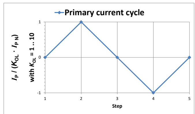
Figure 14: Current cycle used to measure magnetic and electrical offset (transducer supplied)
