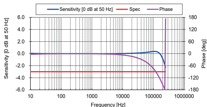
Figure 7: Frequency response
