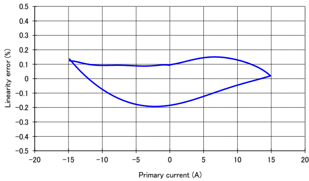
Figure 1: Linearity error
