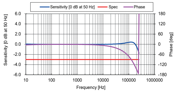
Figure 2: Frequency response
