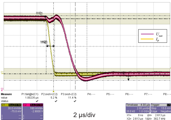
Figure 3: Step response
