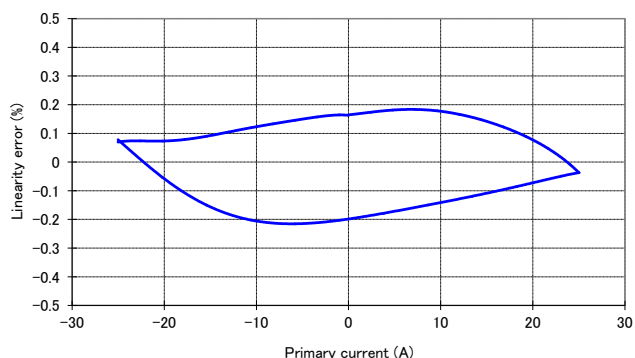
Figure 6: Linearity error
