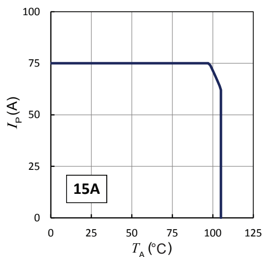
Figures 11 and 12: I_p vs T_A for HO series
