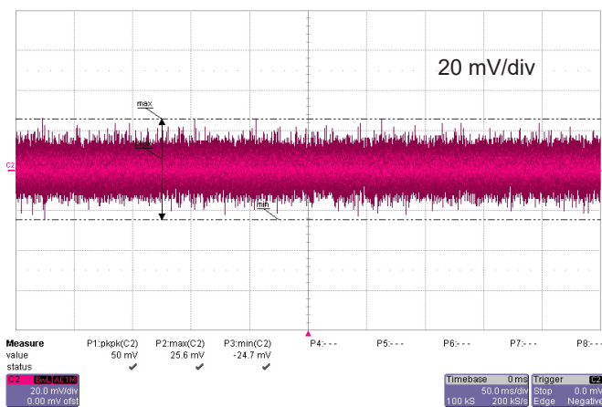
Figure 5: Output noise
