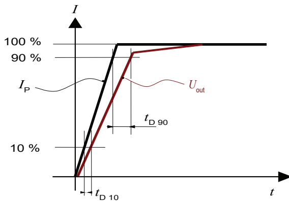
Figure 15: Delay time t_{D90} @ 90 and delay time t_{D10} @ 10
