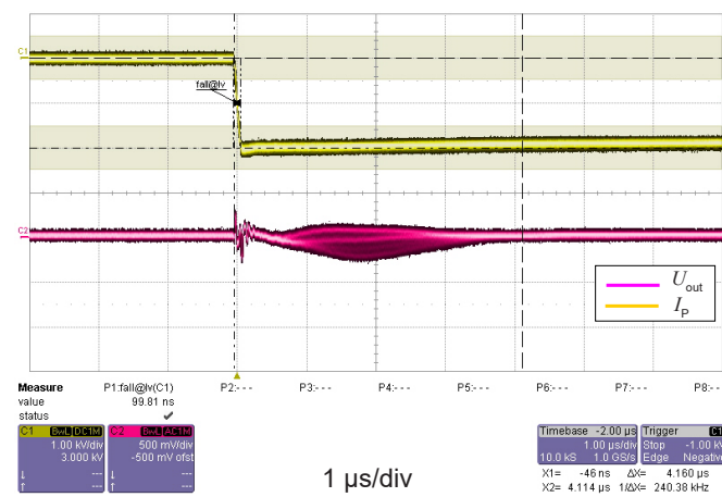
Figure 9: dv/dt
