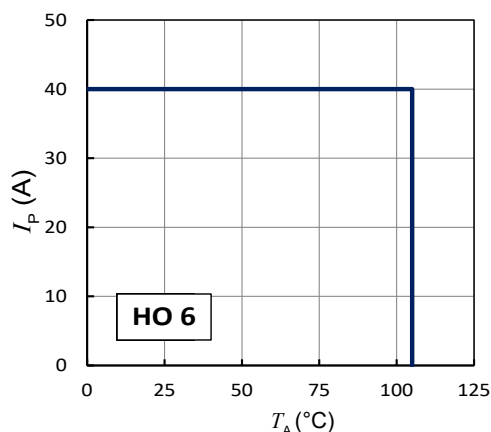
Figure 1: I_p vs T_A for HO series
