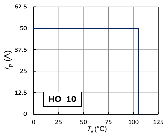
Figure 2: I_p vs T_A for HO series
