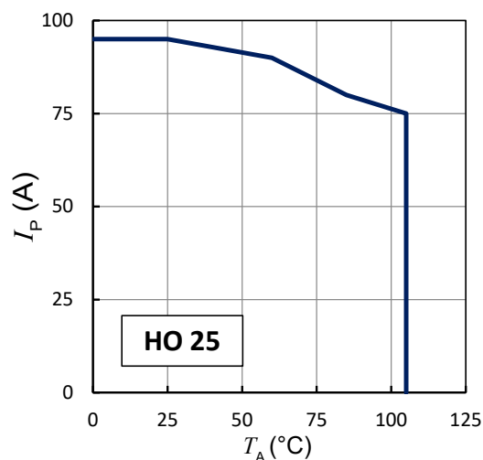
Figure 3: I_p vs T_A for HO series
