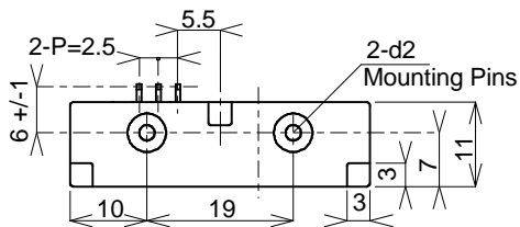
Secondary Pin Identification
