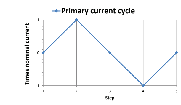
Figure 9: Current cycle used to measure magnetic and electrical offset (transducer supplied)
