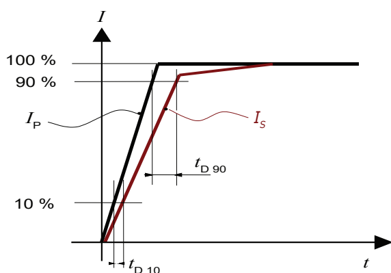
Figure 10: t_{D10} (delay time @ 10 %) and t_{D90} (delay time)
