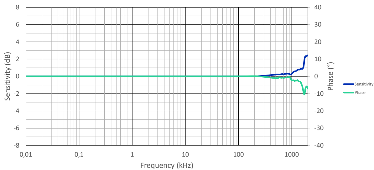
Figure 5: Typical transducer bandwidth response at 25 °C under 1.5 Ω
