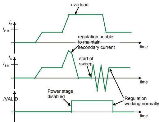
Figure 24: Overload behaviour
