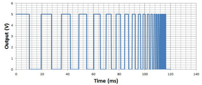
Figure 2: Degauss cycle
