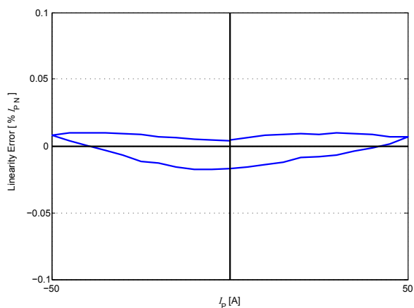
Figure 6: Linearity error
