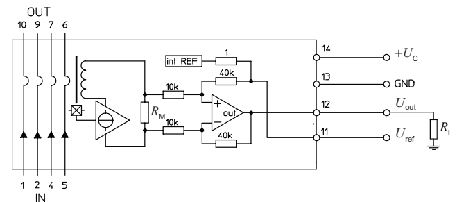
Figure 14: Test connection
