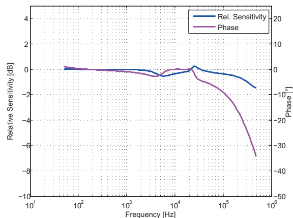
Figure 7: Frequency response
