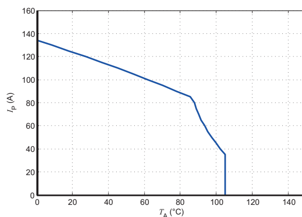
Figure 12: I_P vs T_A for LESR 50-NP/SP1
