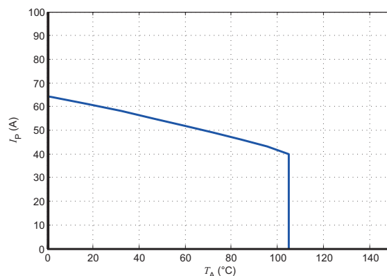
Figure 12: I_P vs T_A for LESR 15-NP/SP1
