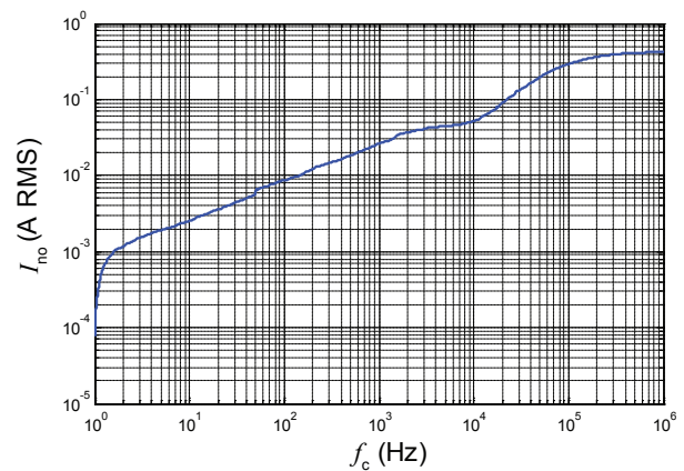
Figure 4: Typical total output noise current with R_M = 100 \Omega (primary referred, RMS)
