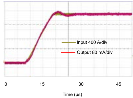
Figure 2: Typical step response (0 to 2 kA, 400 A/μs)
