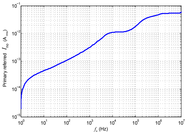
Figure 4: Typical RMS noise current referred to primary with R_M = 10 \text{ } \Omega
