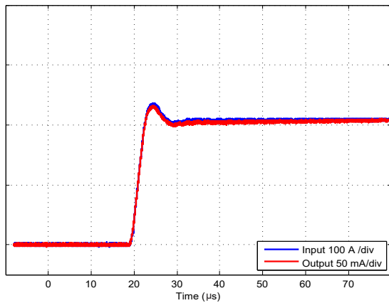
Figure 2: Typical delay time (0 to 200 A, 75 A/μs, with R_M = 10 \text{ } \Omega )
