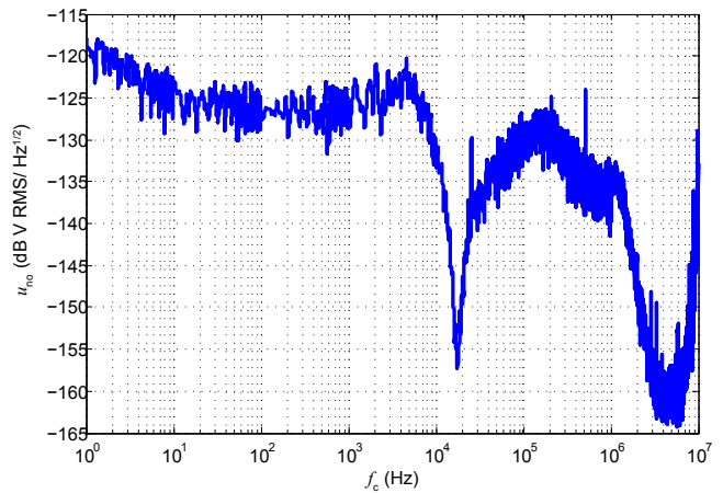
Figure 3: Typical noise voltage spectral density referred to primary u_{no} with R_M = 10 \text{ } \Omega
