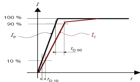
Figure 6: t_{D10} (delay time @ 10 %) and t_{D90} (delay time @ 90 %)
