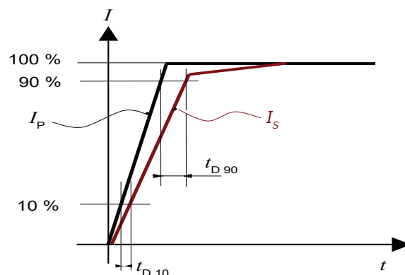
Figure 6: t_{D10} (delay time @ 10 %) and t_{D90} (delay time @ 90 %)
