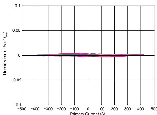
Figure 5: Linearity
