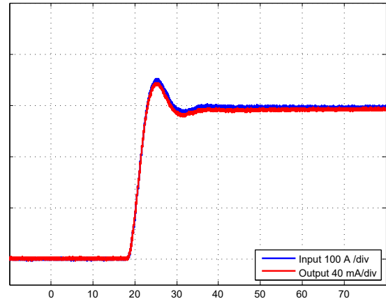
Figure 2: Typical step response (0 to 300 A, 100 A/μs R_M = 10 \Omega )
