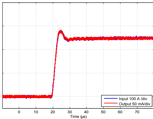
Figure 2: Typical step response (0 to 250 A, 100 A/μs R_M = 10 \Omega )
