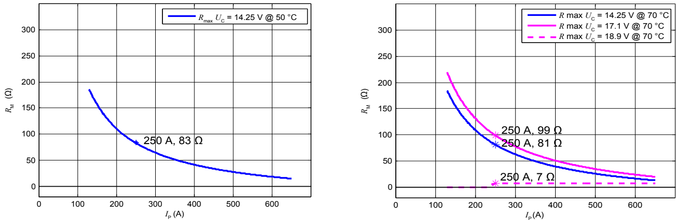
Figure 1: Maximum measuring resistance
