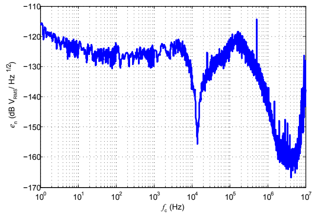
Figure 3: Typical noise voltage spectral density e_n with R_M = 10 \Omega
